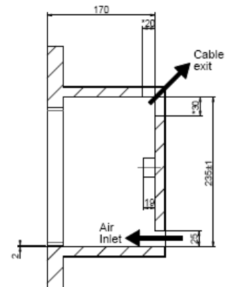
SECTION X-X
